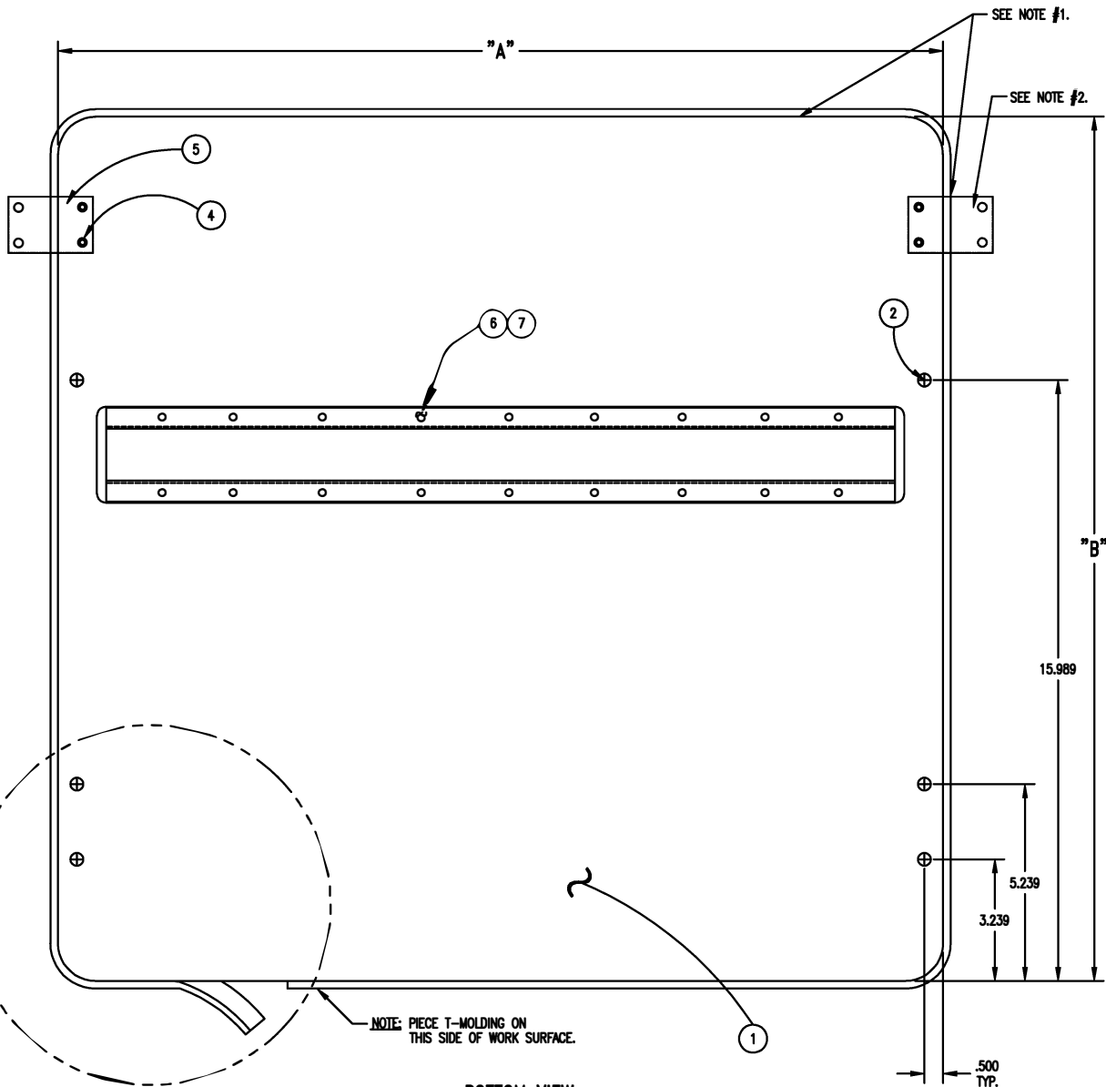
BOTTOM VIEW
